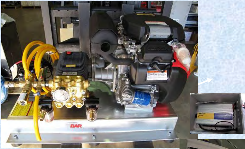
BAR4527G-HEB Gear Box Drive 4500 Psi 15 l/min. Gear Box Drive on base Plate with Invertor Honda 27Hp, Comet TW5550 Pump Trade Price $poa
